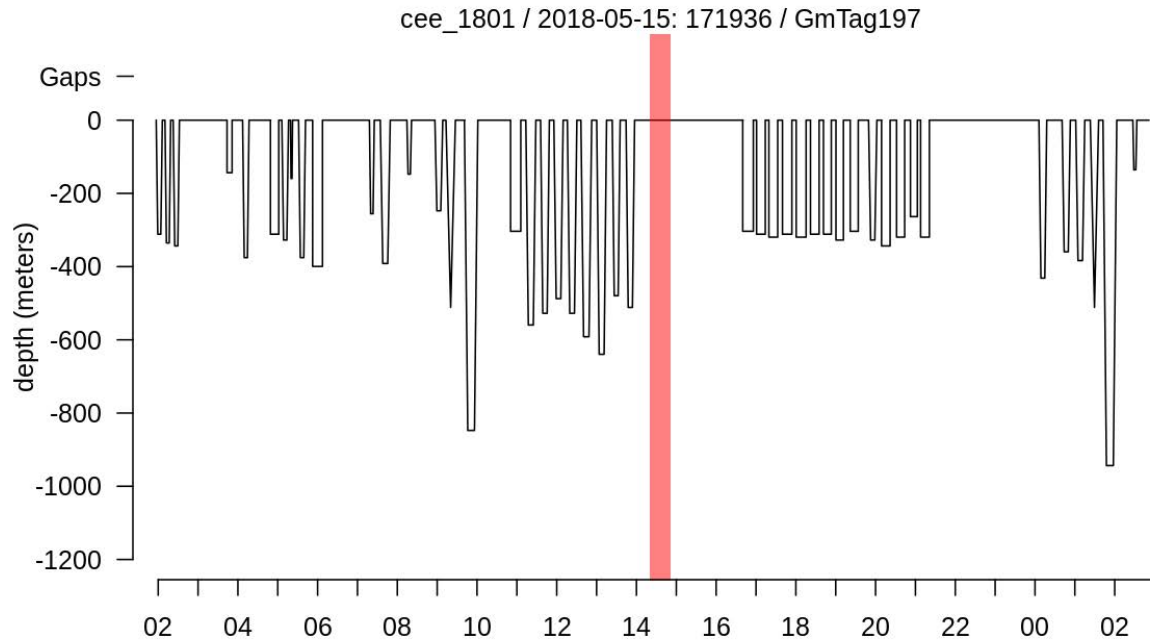
Figure 9. Available dive data for focal whale Gm197 before, during, and after Atlantic-BRS CEE# 18-01
