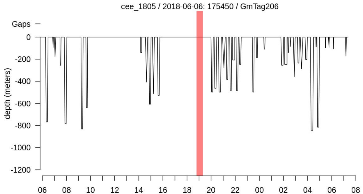
3 4 Figure 85. Available dive data for whale Gm206 before, during, and after Atlantic-BRS CEE# 18-05
