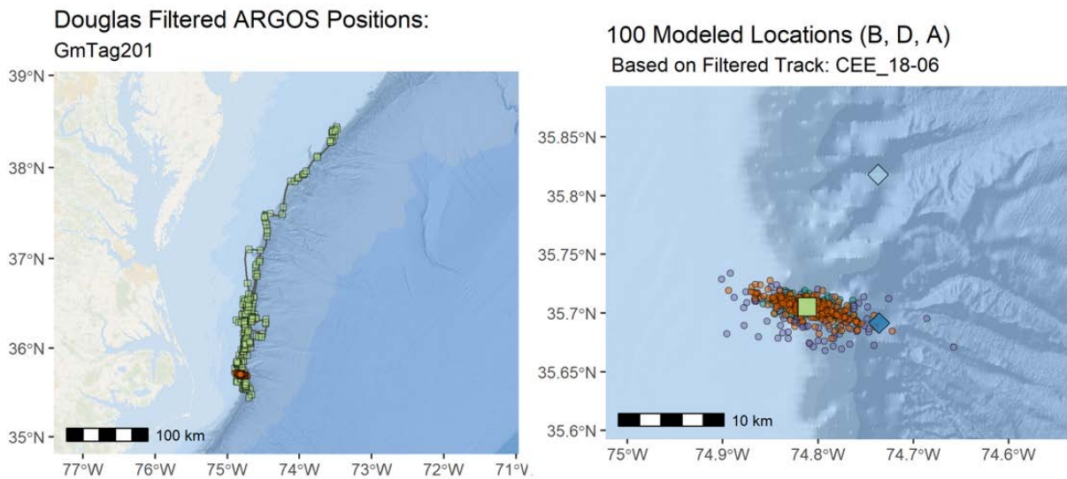
Figure 92. Estimated surface positions for focal whale Gm201 before, during, and after Atlantic-BRS CEE# 18-06
