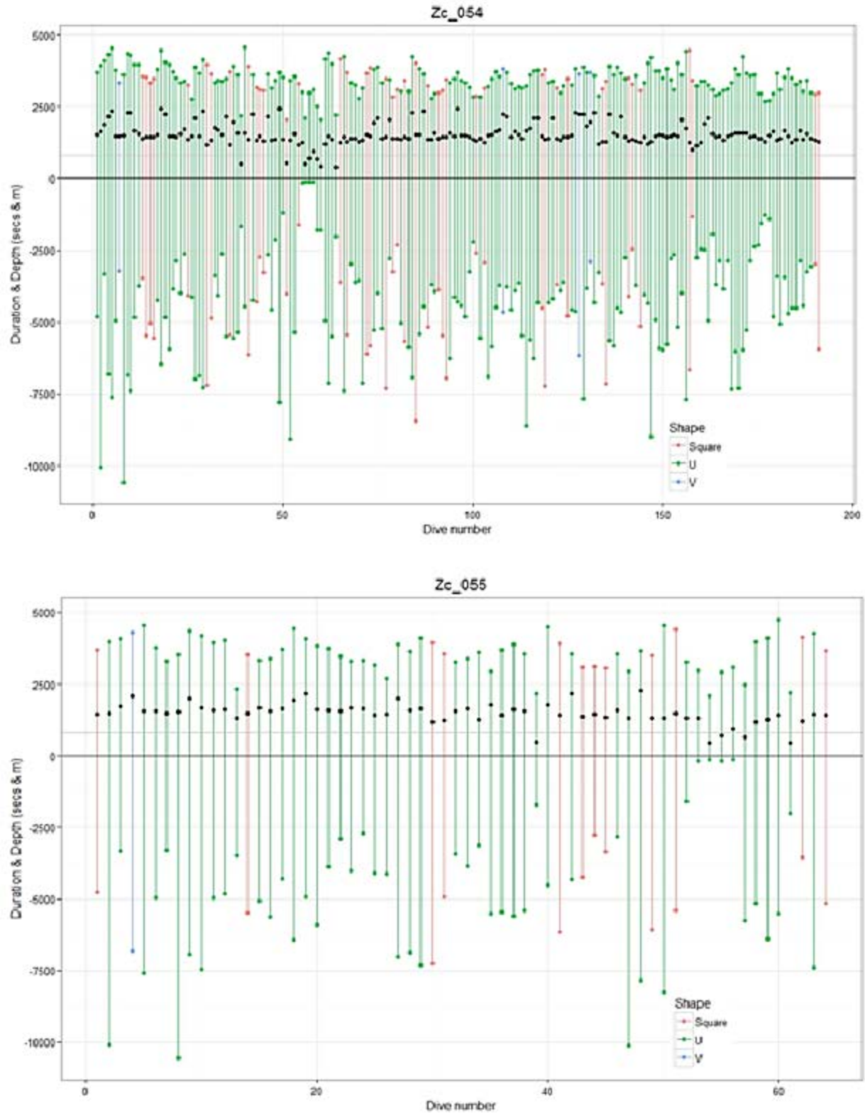
1 Figure 167. Plots of continuous dive samples for two baseline tags, showing cyclic nature of 2 variables. Each line shows dive duration above the x-axis with following inter deep dive interval 3 below the x-axis. Black dots show dive depth. Lines colored by shape.
