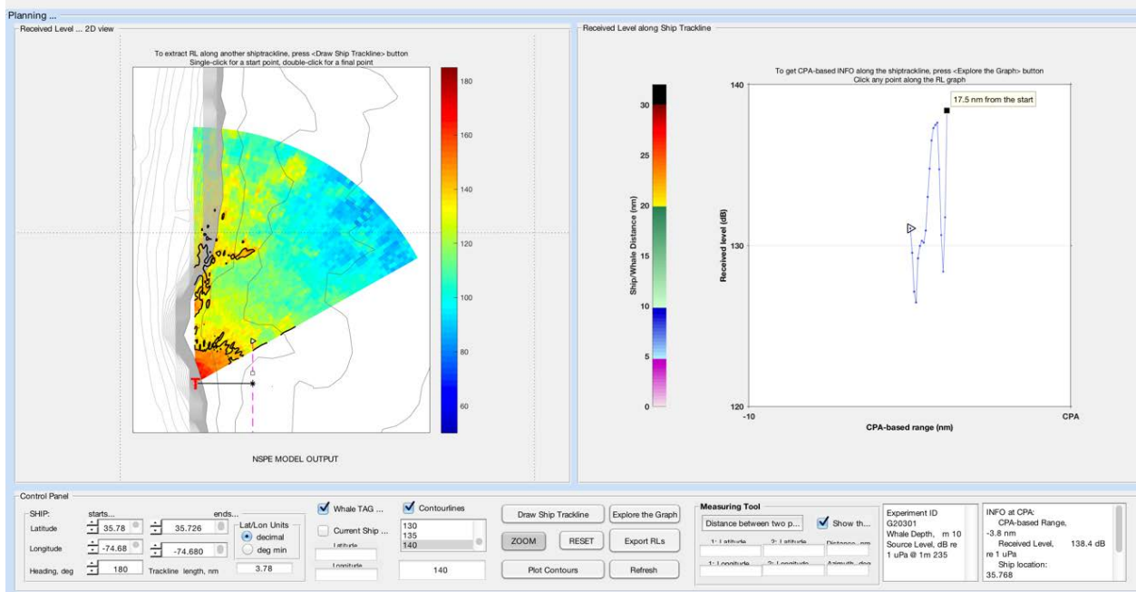
Figure 89. RL model prediction at 10 m depth for focal whale Gm203 for Atlantic-BRS CEE# 18-06 (END position of USS RAMAGE)
