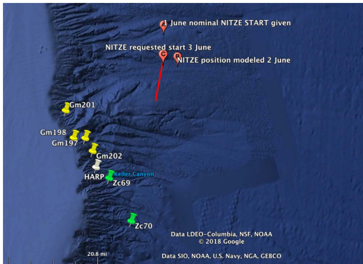
Figure 40. Map showing animal positions and initial and final requested positions of USS NITZE for Atlantic-BRS CEE# 18-04 on 3 June 2018
