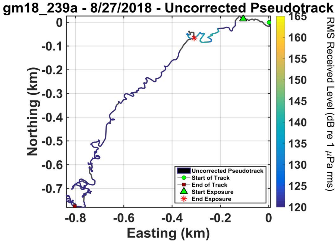
1 Figure 131. Uncorrected pseudotrack based on surface positions and tag data for focal whale 2 Gm18_239a (DTAG) before, during, and after Atlantic-BRS CEE# 18-08
