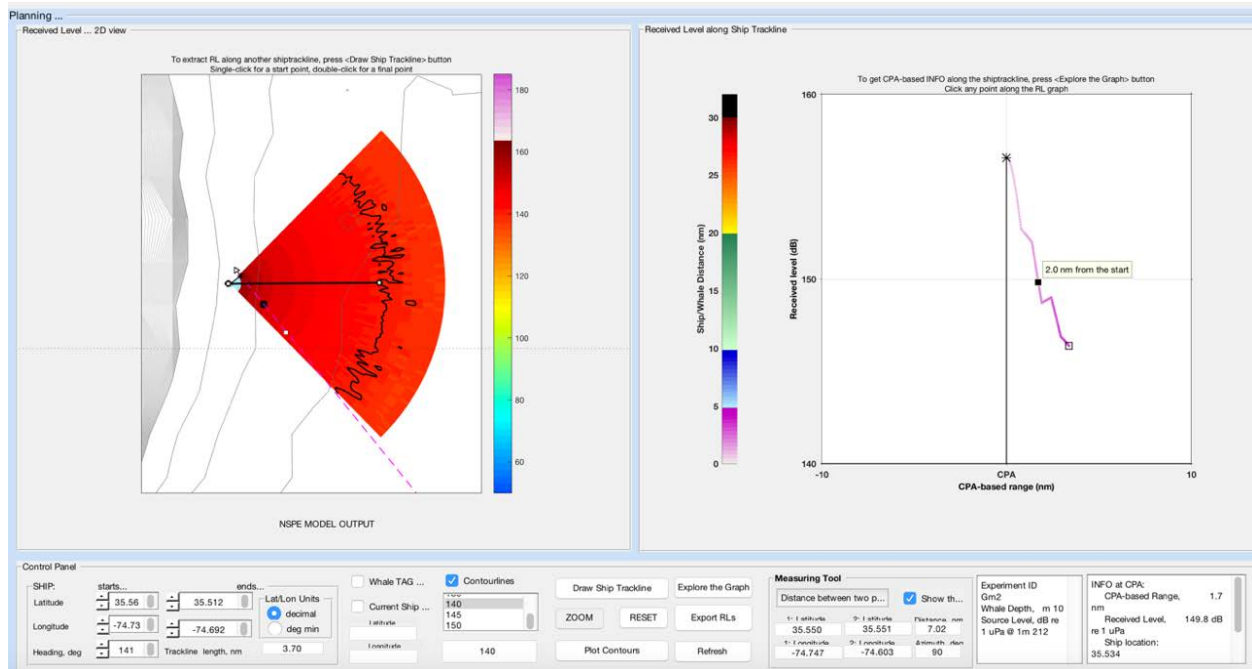
1 Figure 129. RL model prediction at 10 m depth for focal whale Gm18_239a for Atlantic-BRS CEE# 2 18-08
