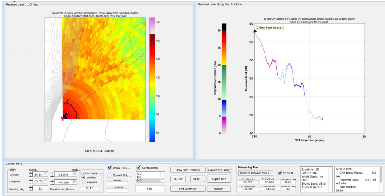
Figure 8. Estimated surface positions for focal whale Gm197 before, during, and after Atlantic-BRS CEE# 18-01
