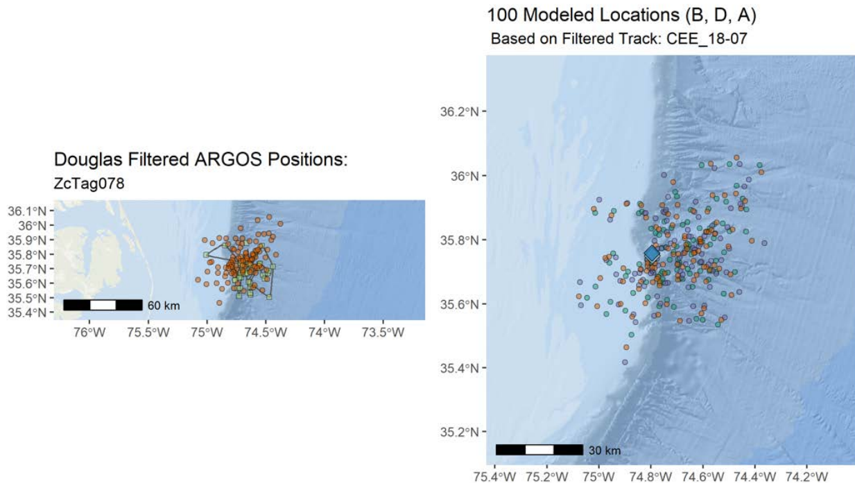
3 4 Figure 114. Estimated surface positions for whale Zc78 before, during, and after Atlantic-BRS 5 CEE# 18-07
